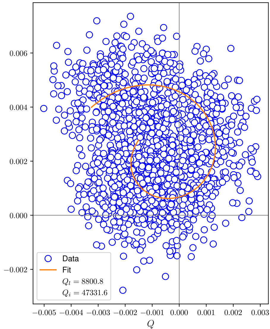
I-Q Plot
