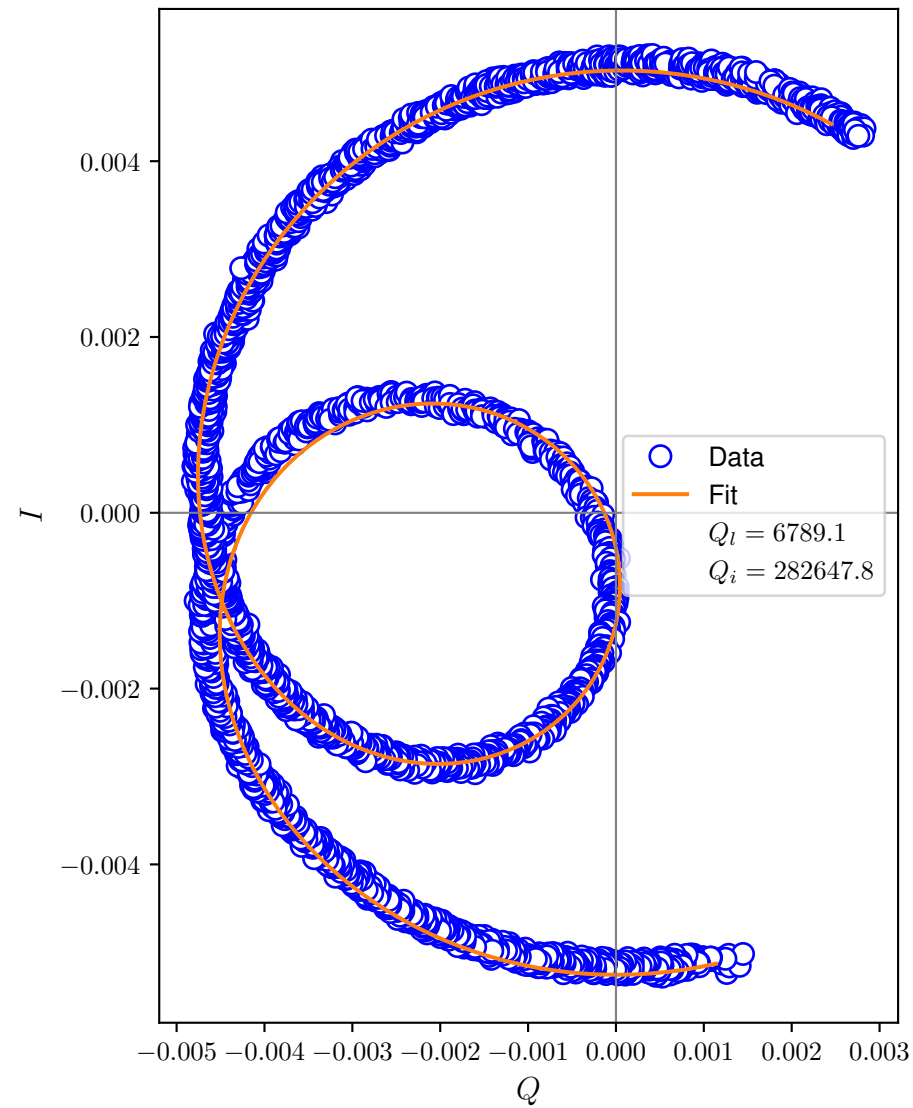
I-Q Plot
