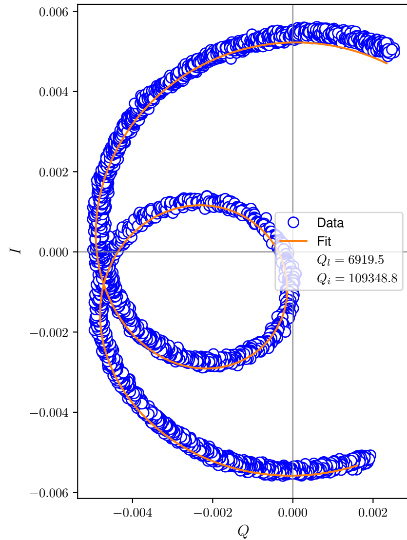
I-Q Plot
