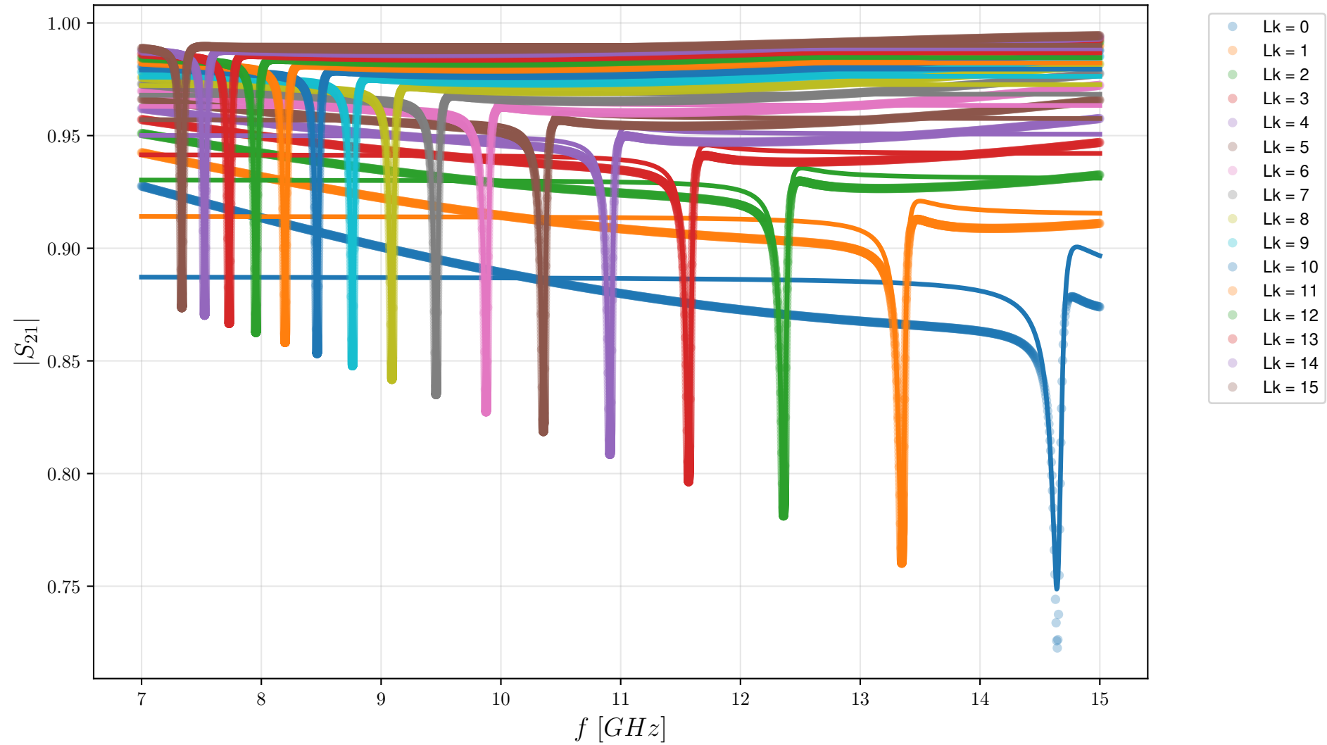
Resonances at different Kinetic Inductances ( L_k )
