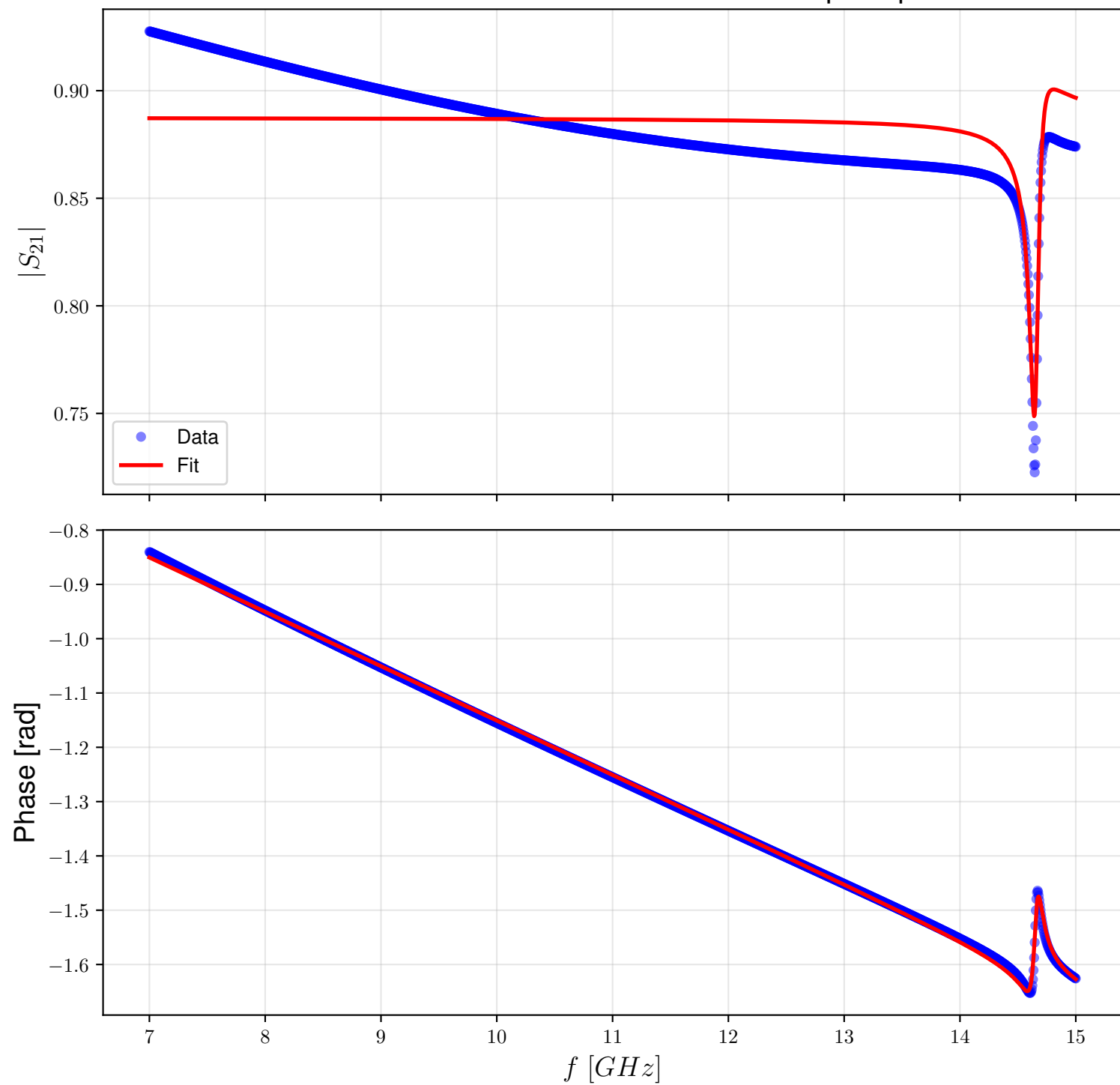
Resonance Fit - Kinetic Inductance: 0 pH/sq
