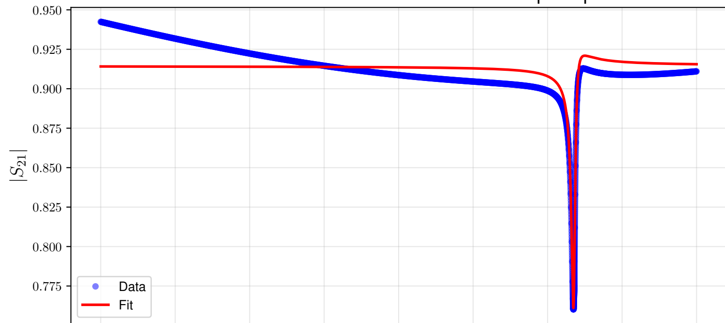
Resonance Fit - Kinetic Inductance: 1 pH/sq
