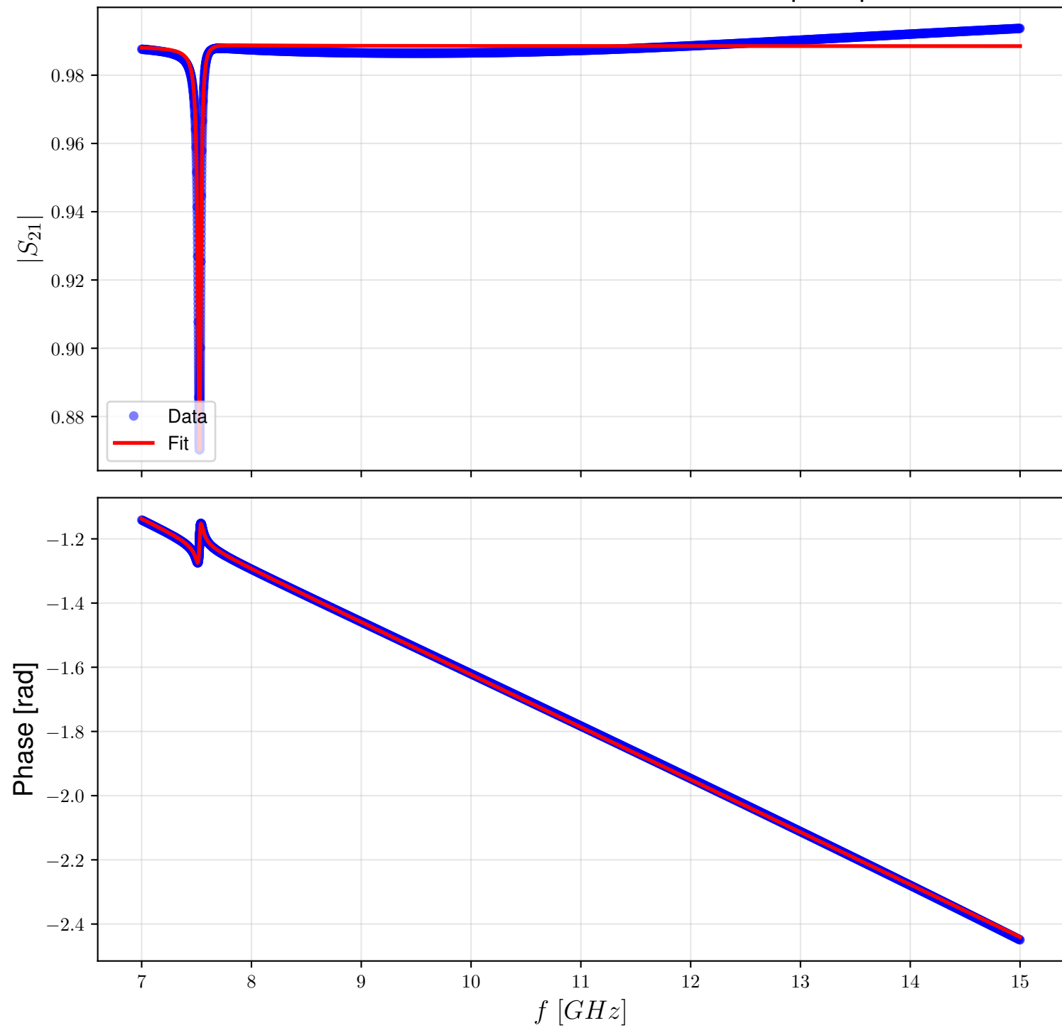
Resonance Fit - Kinetic Inductance: 14 pH/sq
