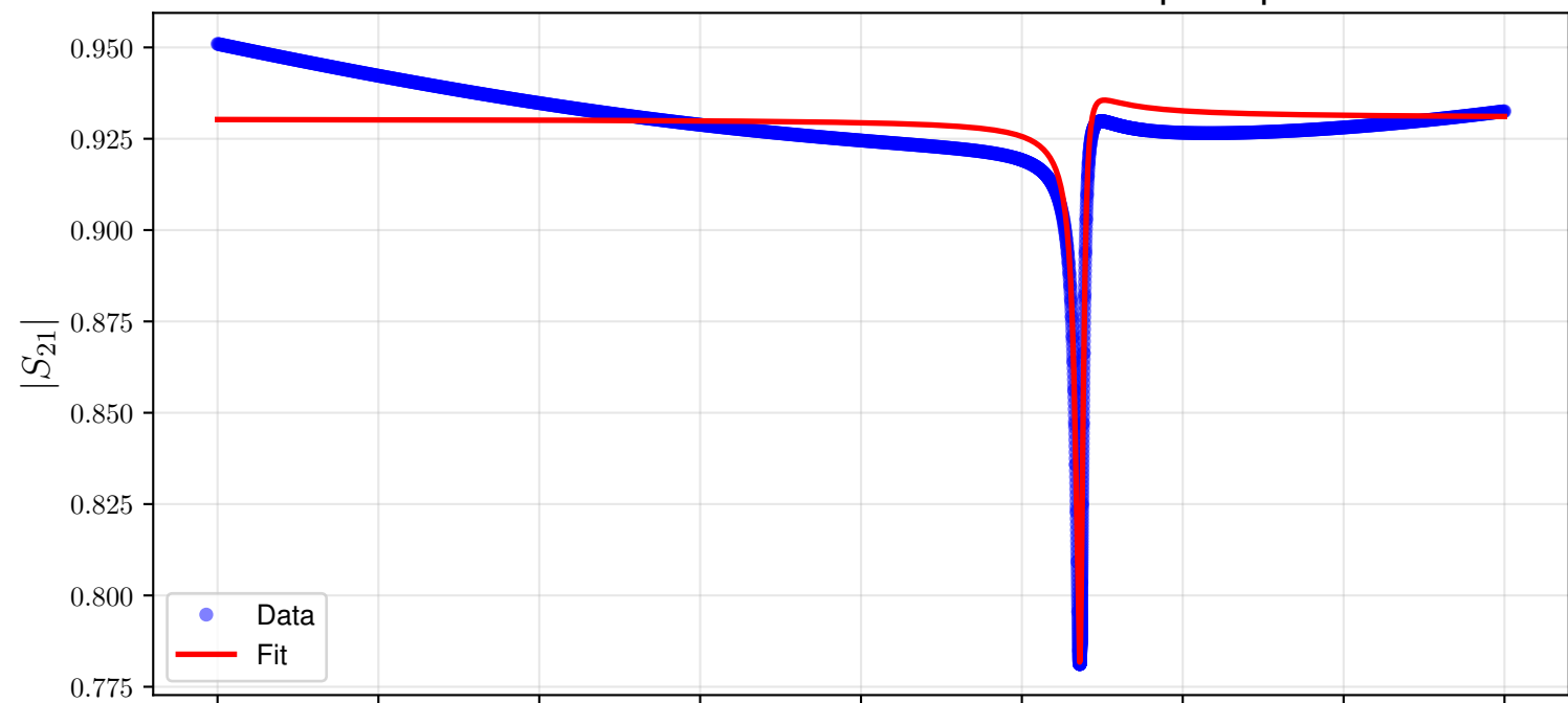
Resonance Fit - Kinetic Inductance: 2 pH/sq
