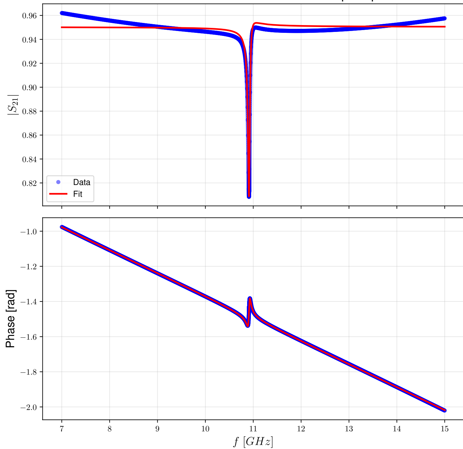
Resonance Fit - Kinetic Inductance: 4 pH/sq
