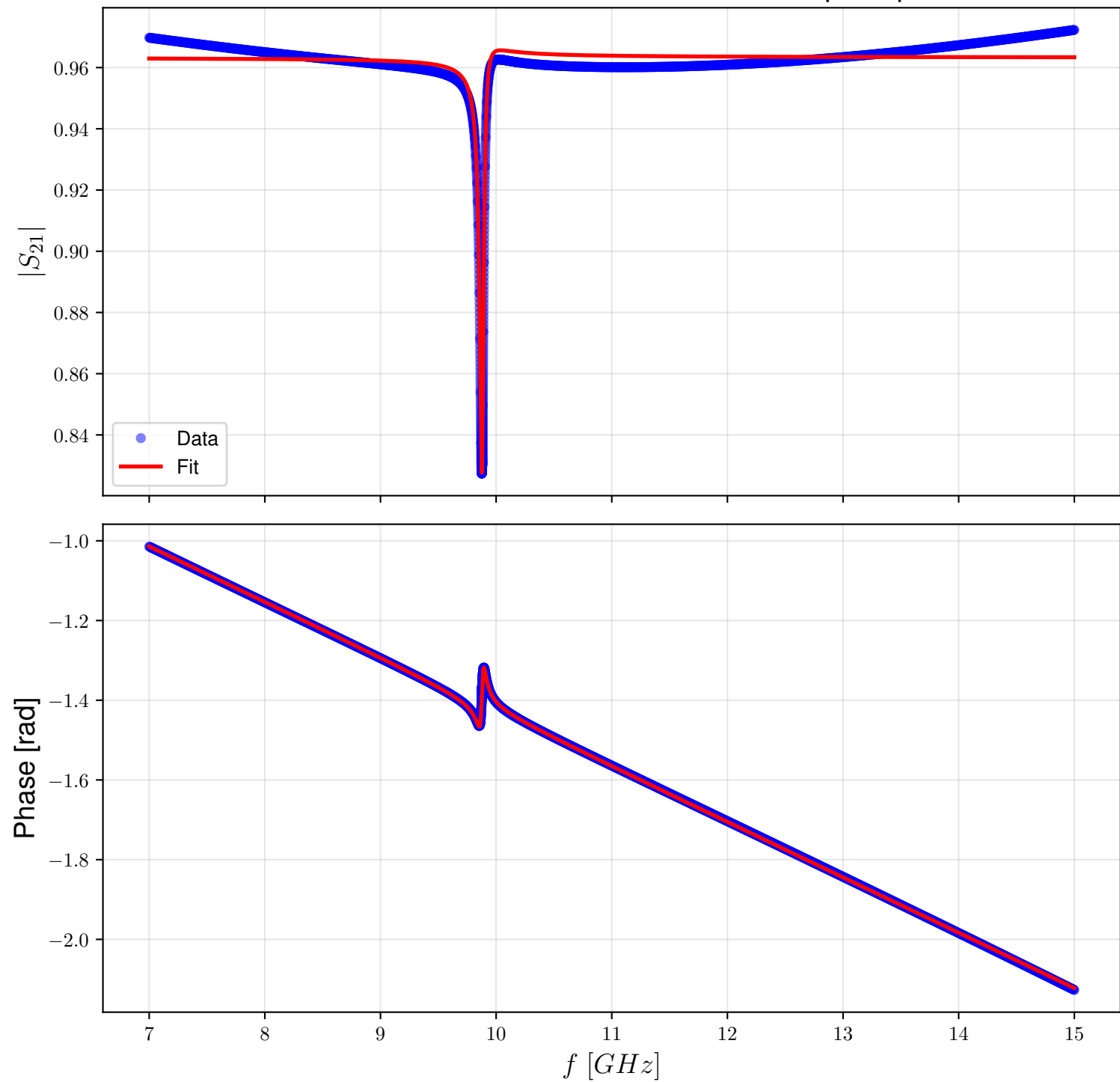
Resonance Fit - Kinetic Inductance: 6 pH/sq
