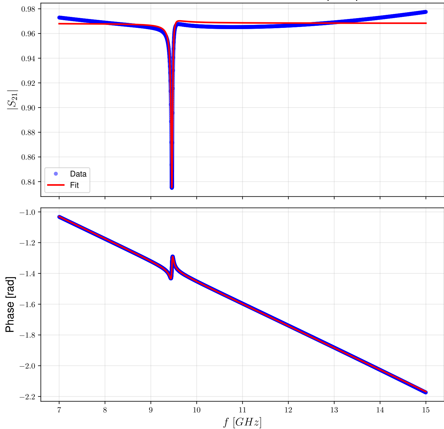
Resonance Fit - Kinetic Inductance: 7 pH/sq
