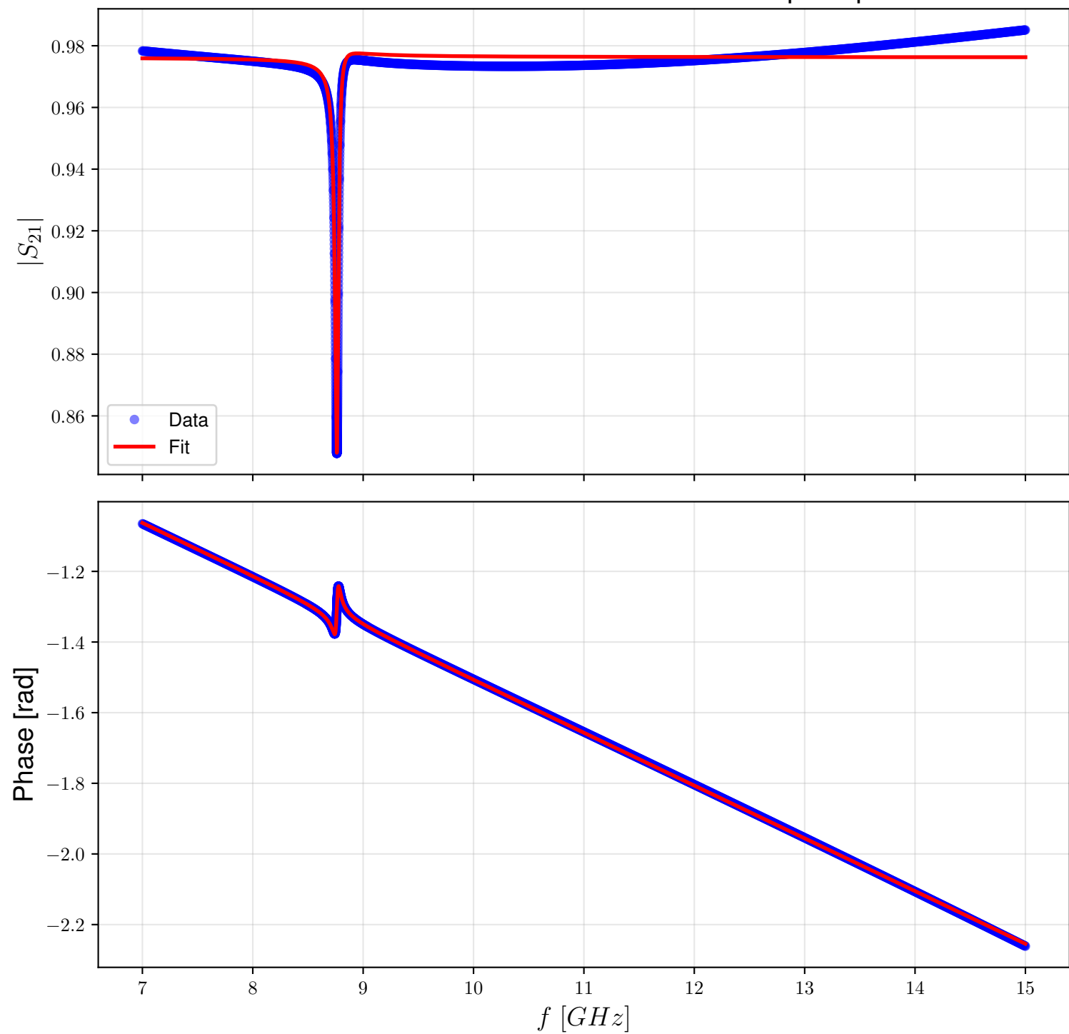
Resonance Fit - Kinetic Inductance: 9 pH/sq
