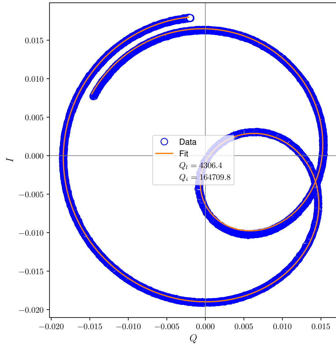
I-Q Plot
