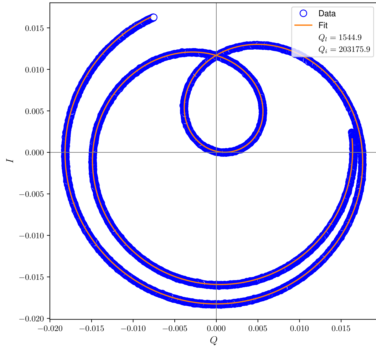
I-Q Plot
