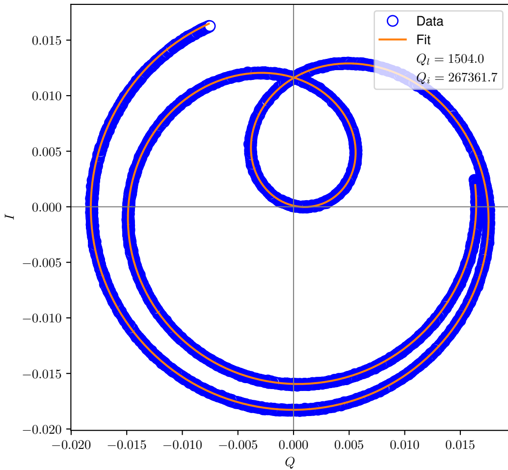
I-Q Plot
