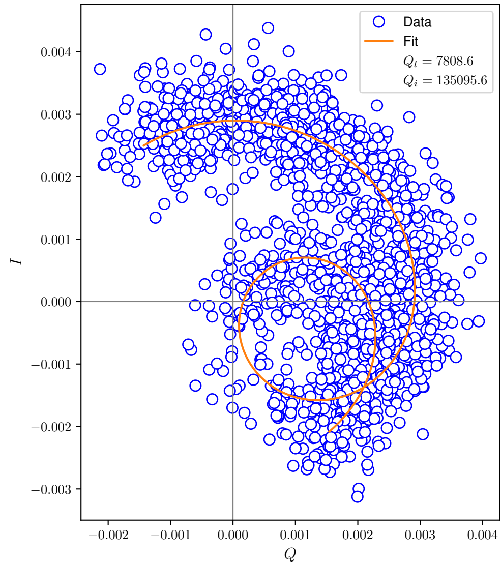
I-Q Plot
