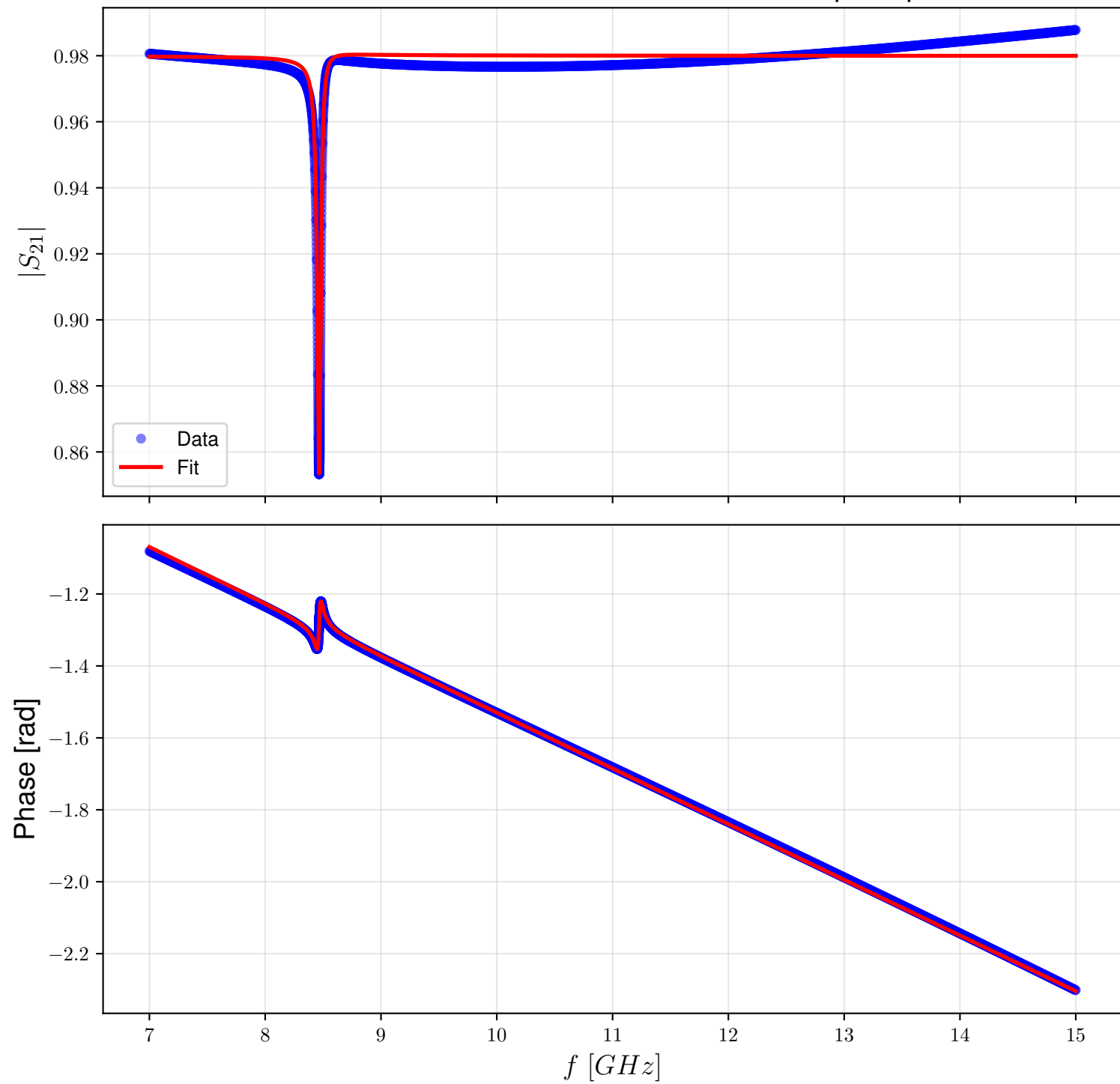
Resonance Fit - Kinetic Inductance: 10 pH/sq
