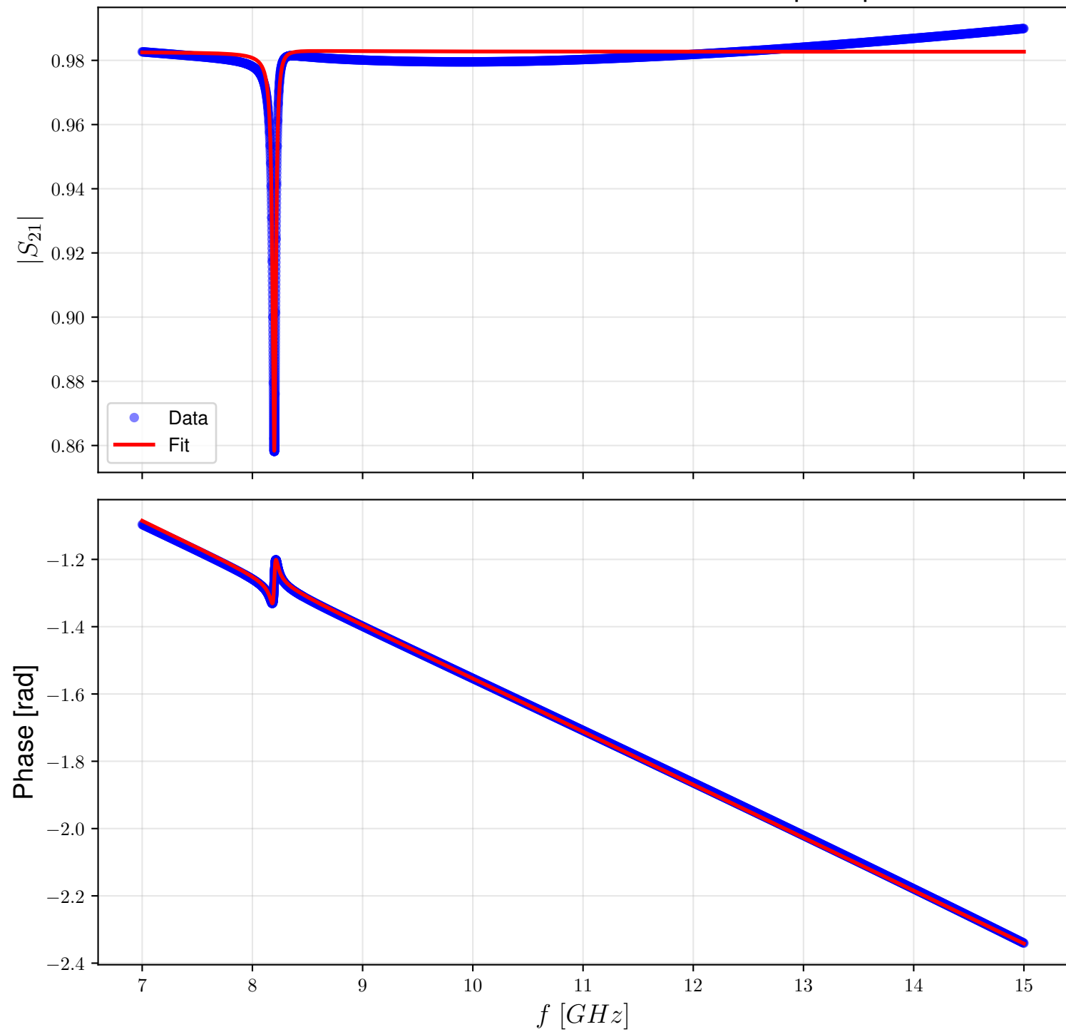
Resonance Fit - Kinetic Inductance: 11 pH/sq
