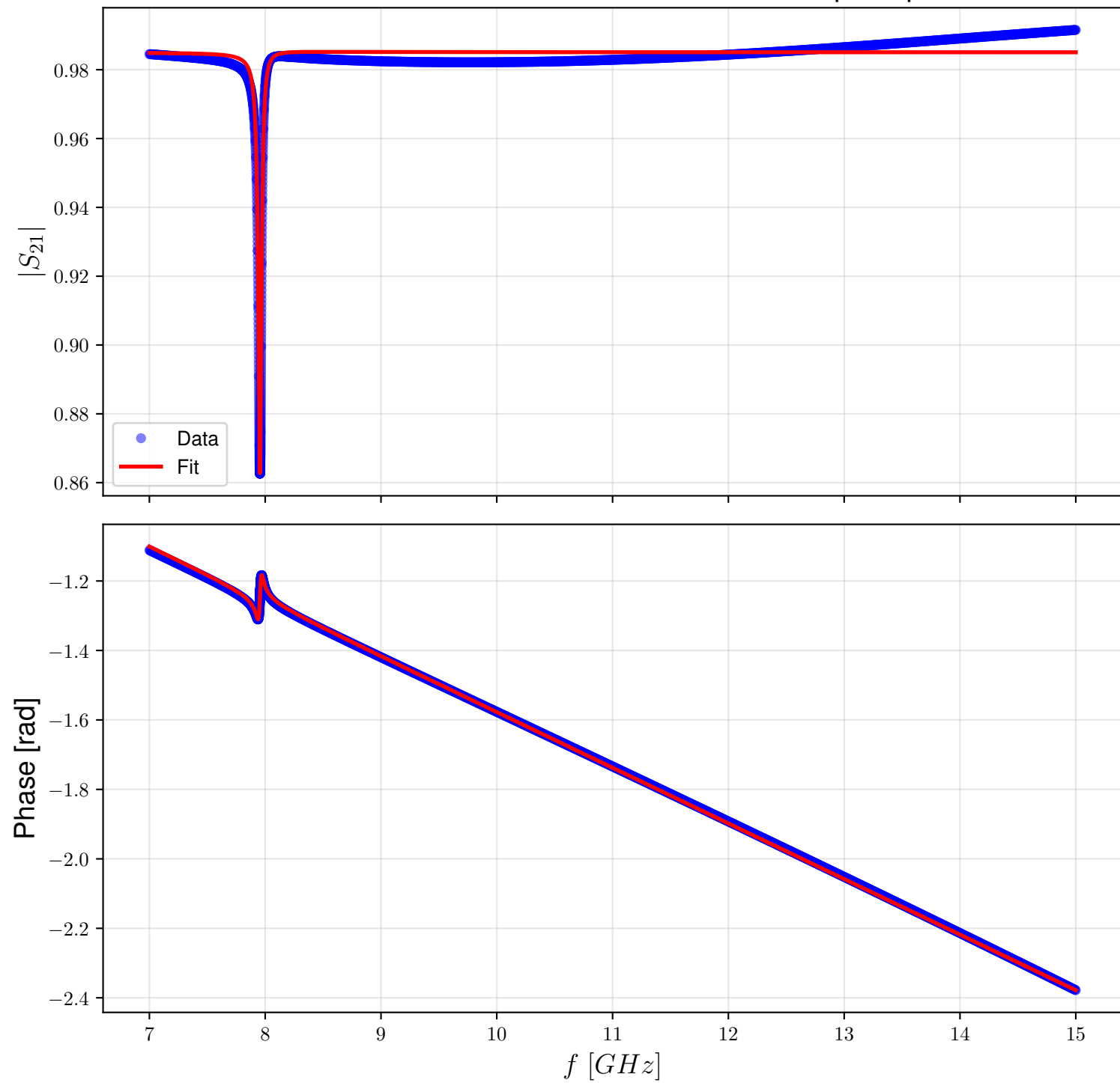
Resonance Fit - Kinetic Inductance: 12 pH/sq
