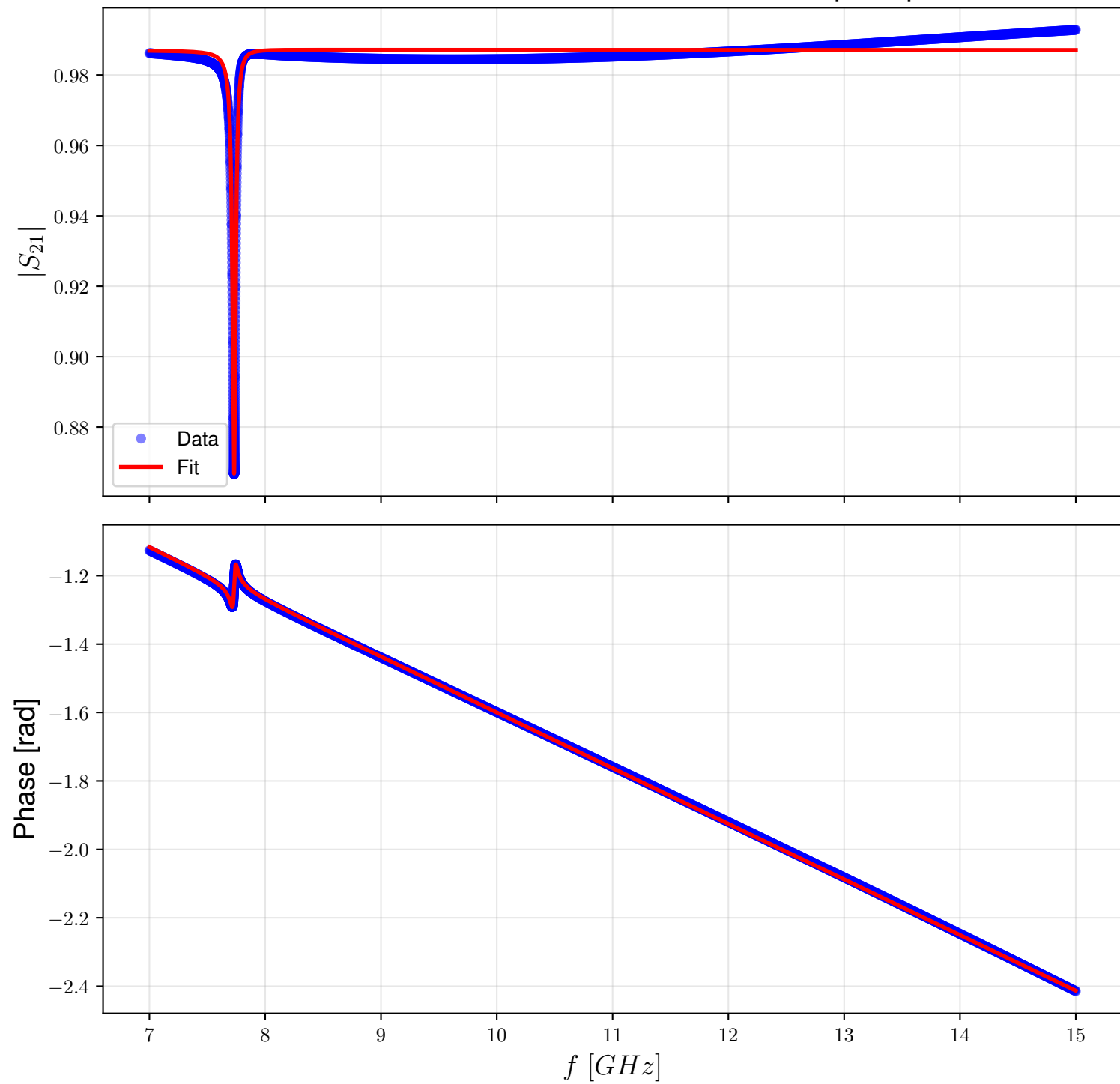
Resonance Fit - Kinetic Inductance: 13 pH/sq
