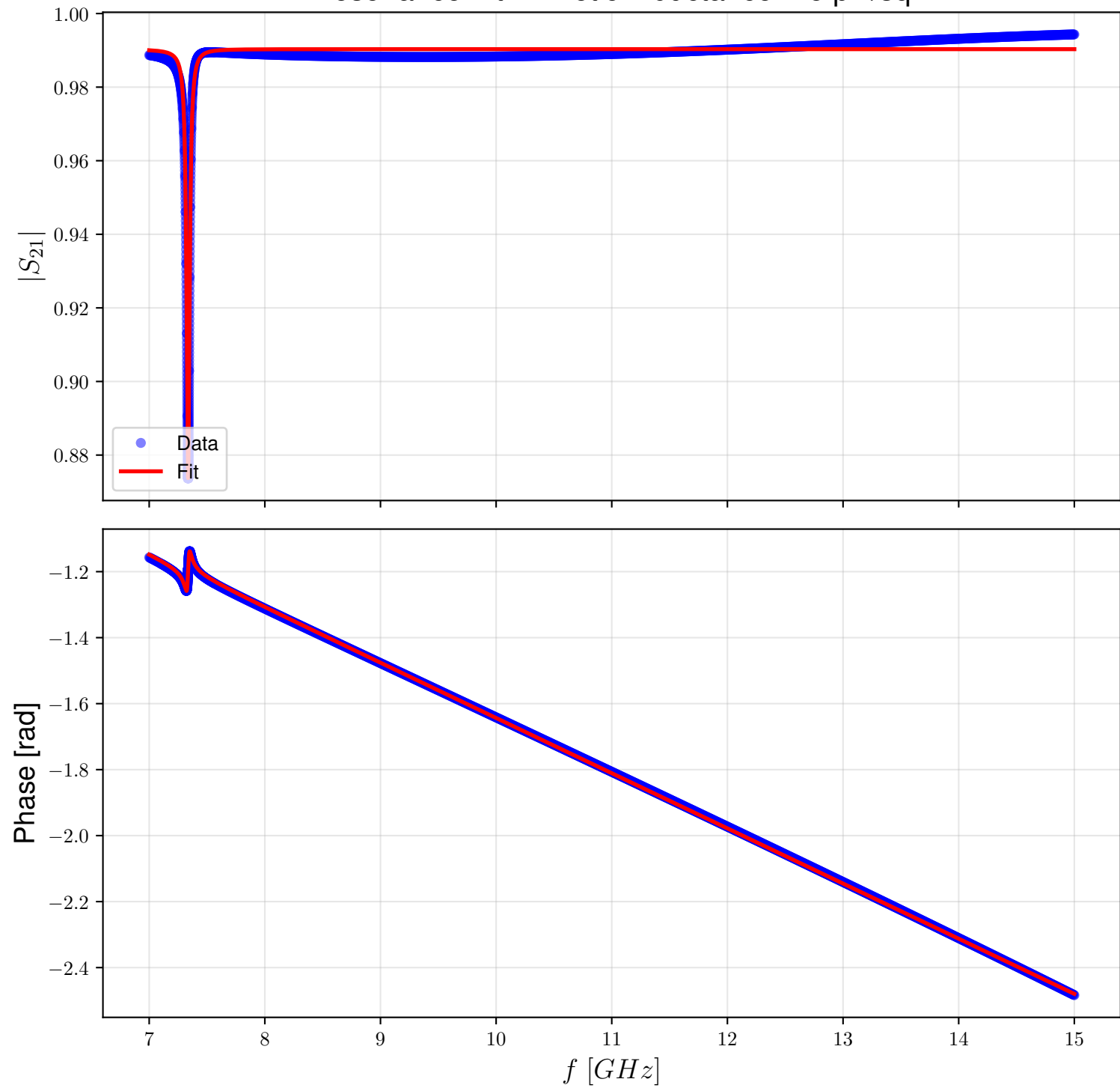
Resonance Fit - Kinetic Inductance: 15 pH/sq
