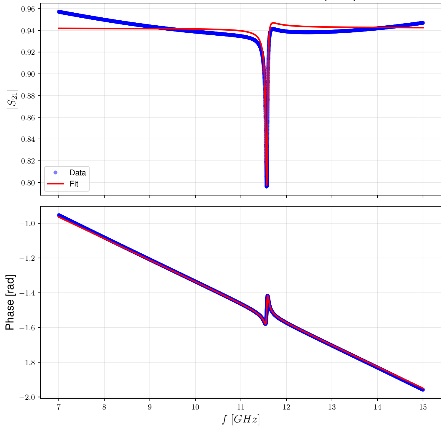
Resonance Fit - Kinetic Inductance: 3 pH/sq
