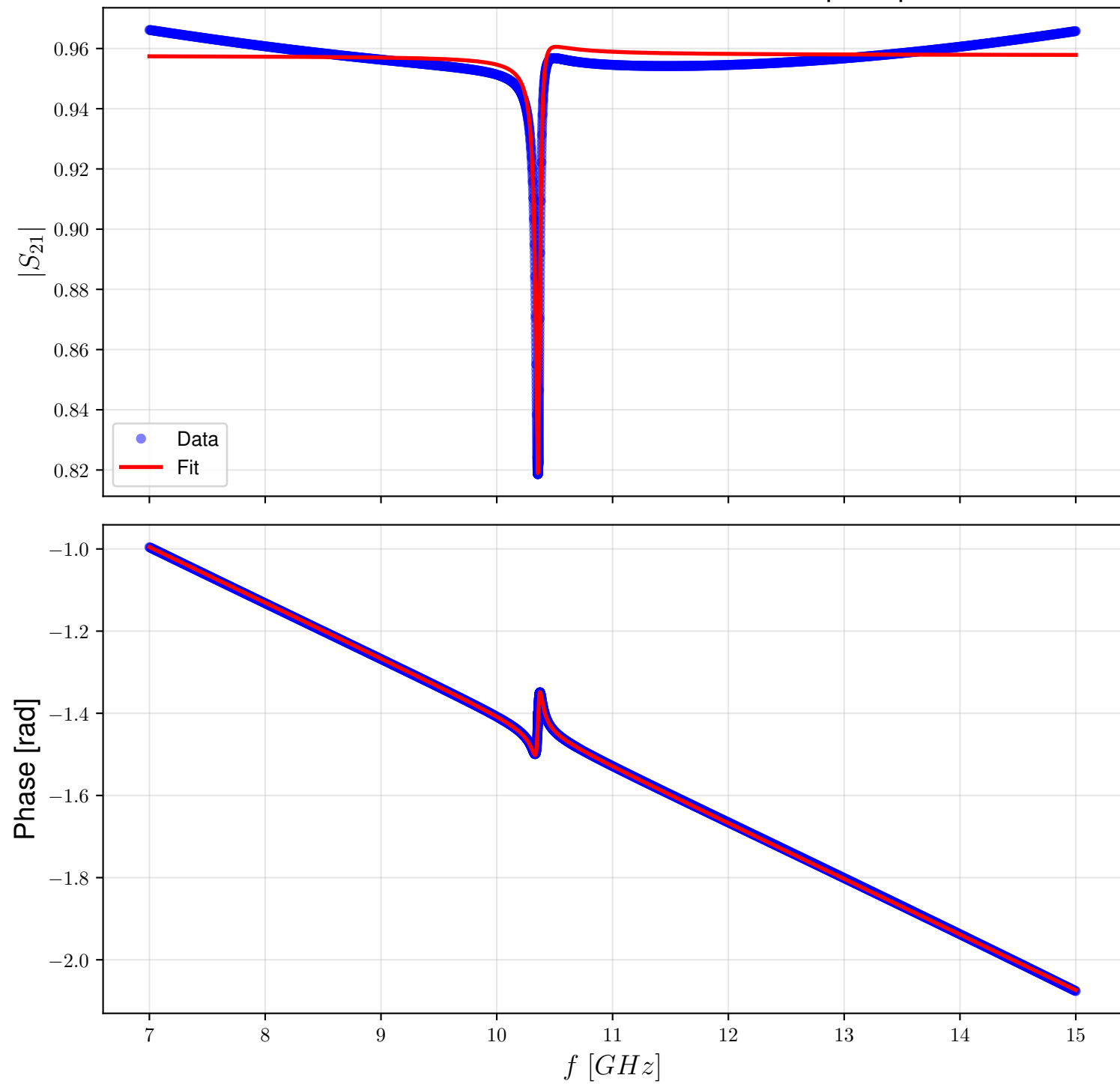
Resonance Fit - Kinetic Inductance: 5 pH/sq
