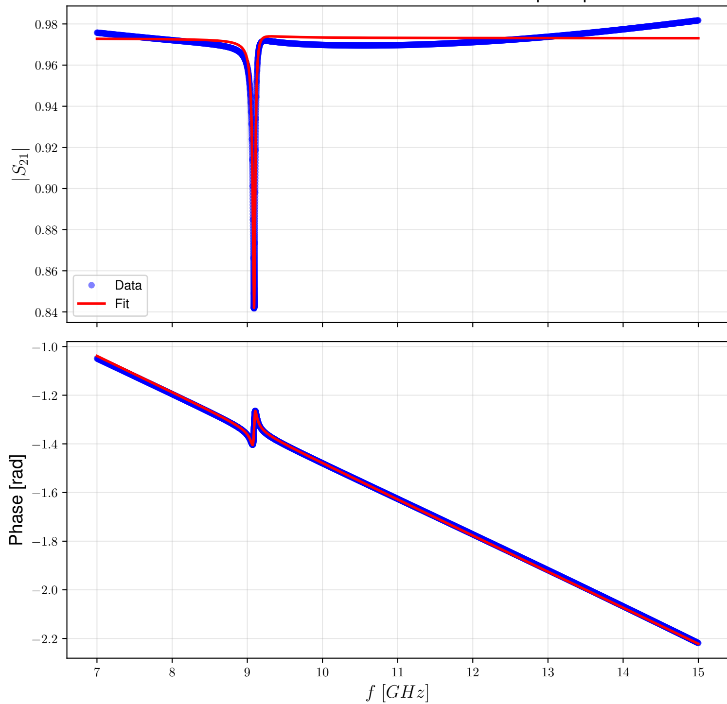
Resonance Fit - Kinetic Inductance: 8 pH/sq
