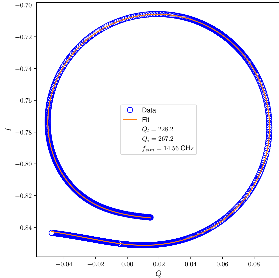
I-Q Plot
