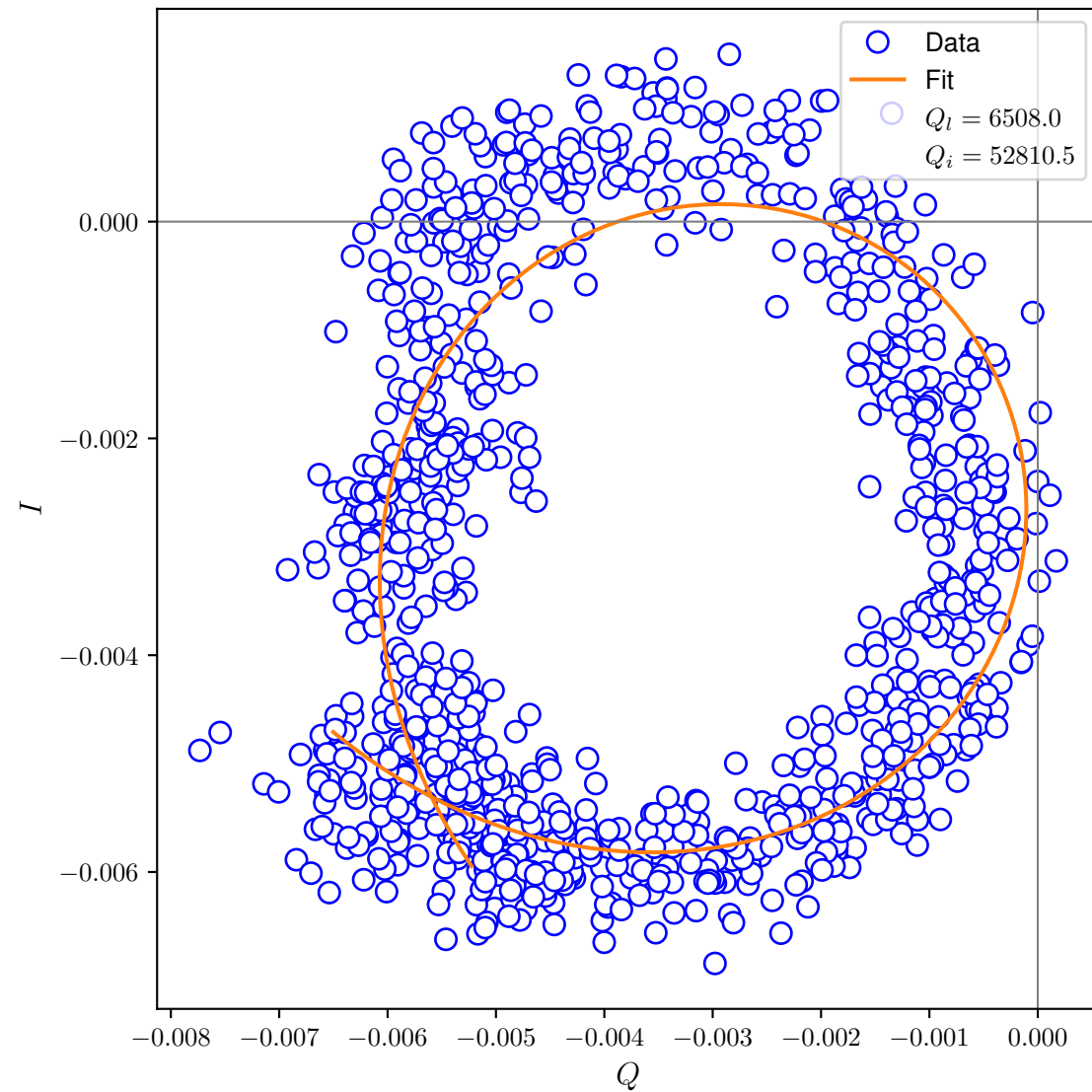
I-Q Plot
