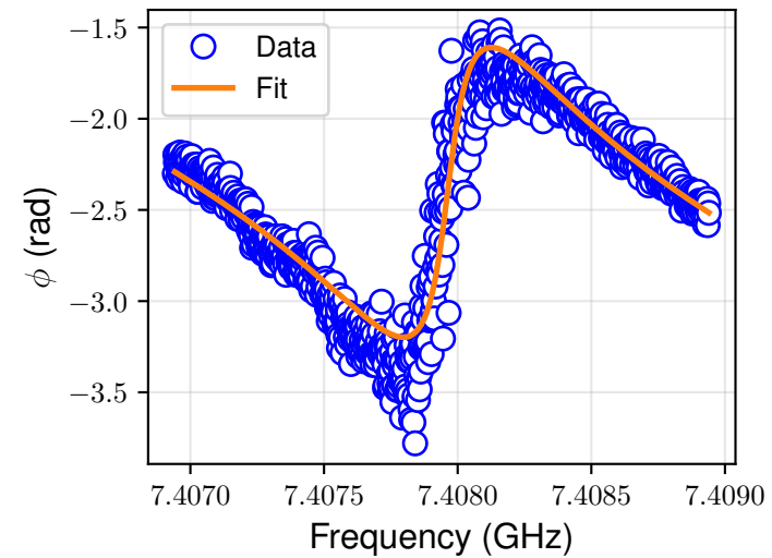
Phase
