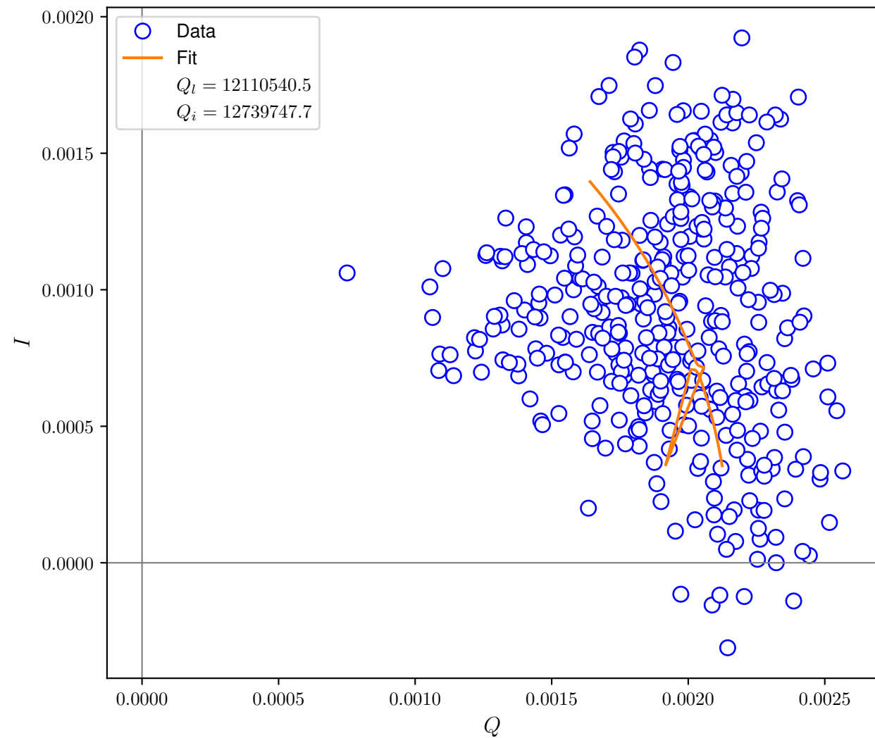
I-Q Plot
