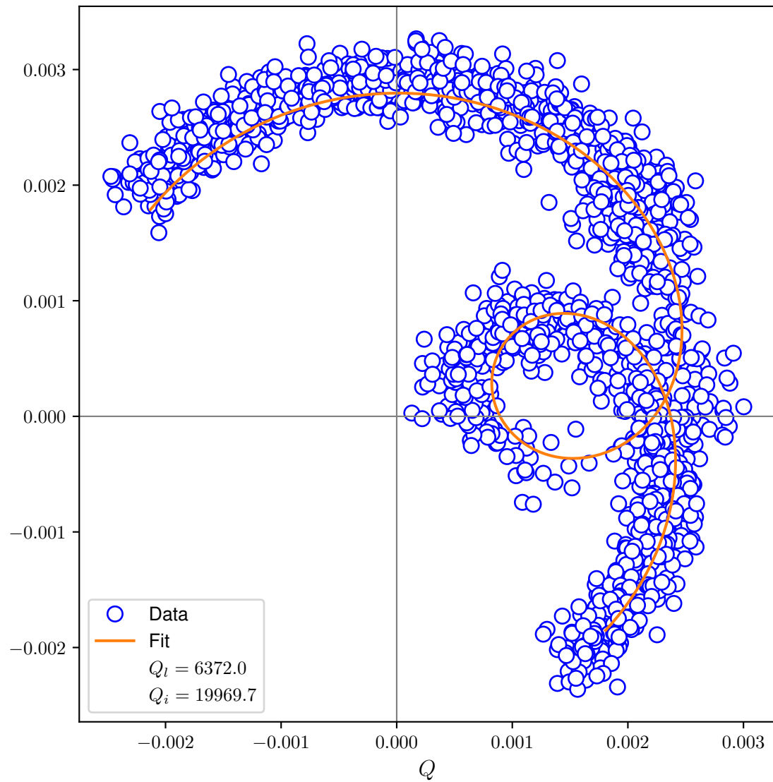
I-Q Plot
