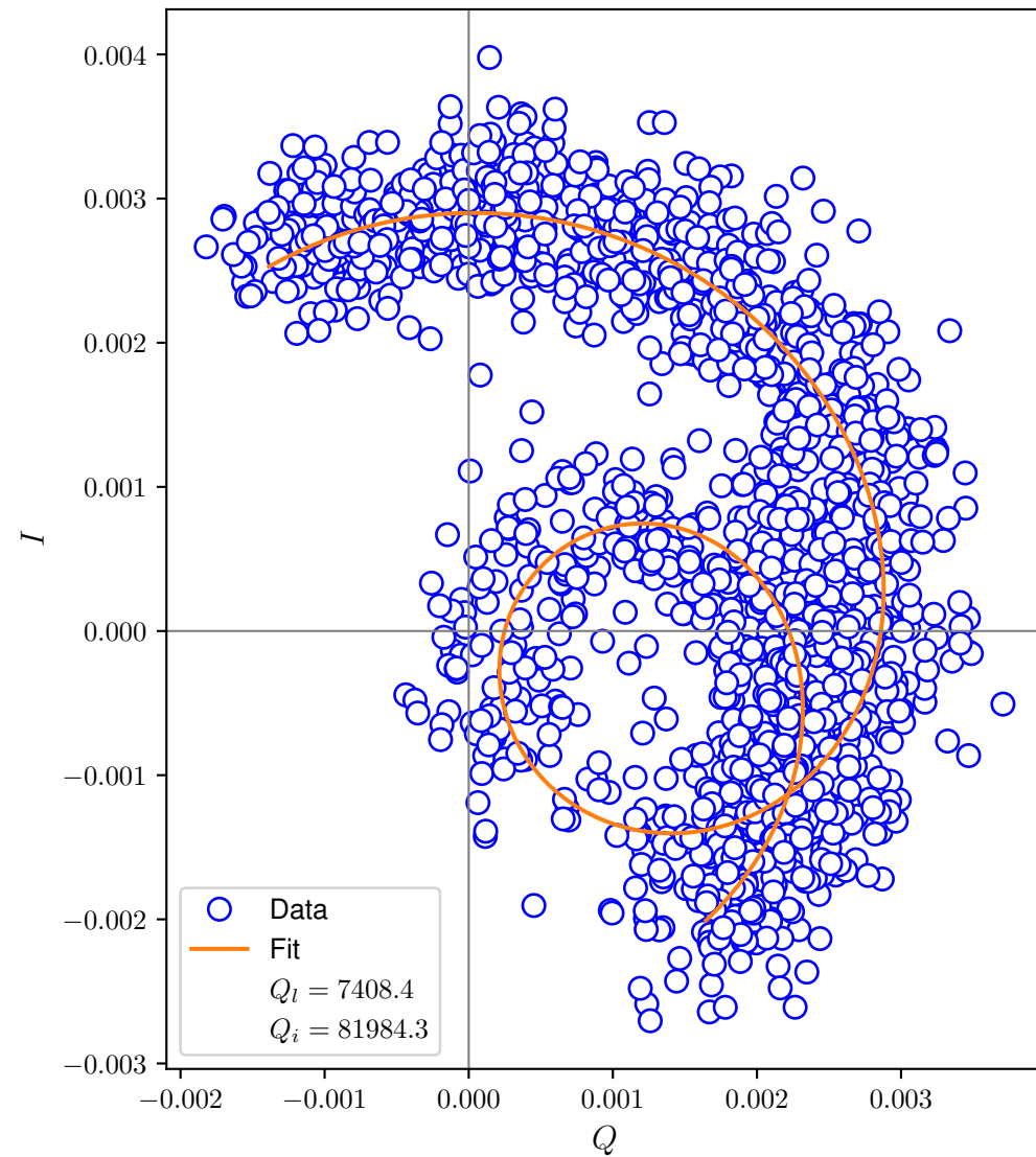
I-Q Plot
