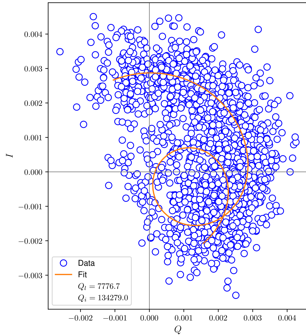
I-Q Plot
