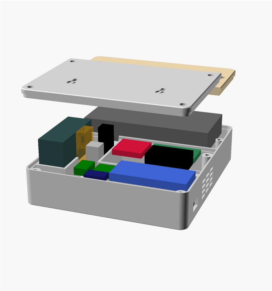
Exploded: front shell, modules, battery door, lid
