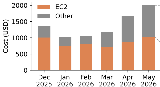
AWS cost, aggregated by "service"
