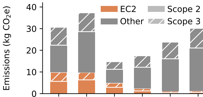
AWS reported emissions by "service"
