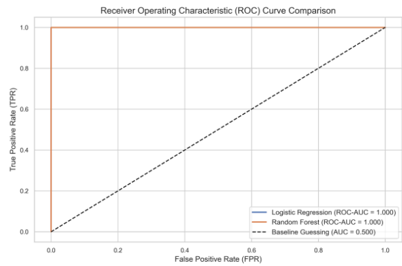
Figure 5: ROC Curve Comparison
