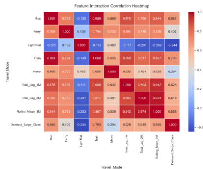
Figure 2: Feature Correlation Matrix
