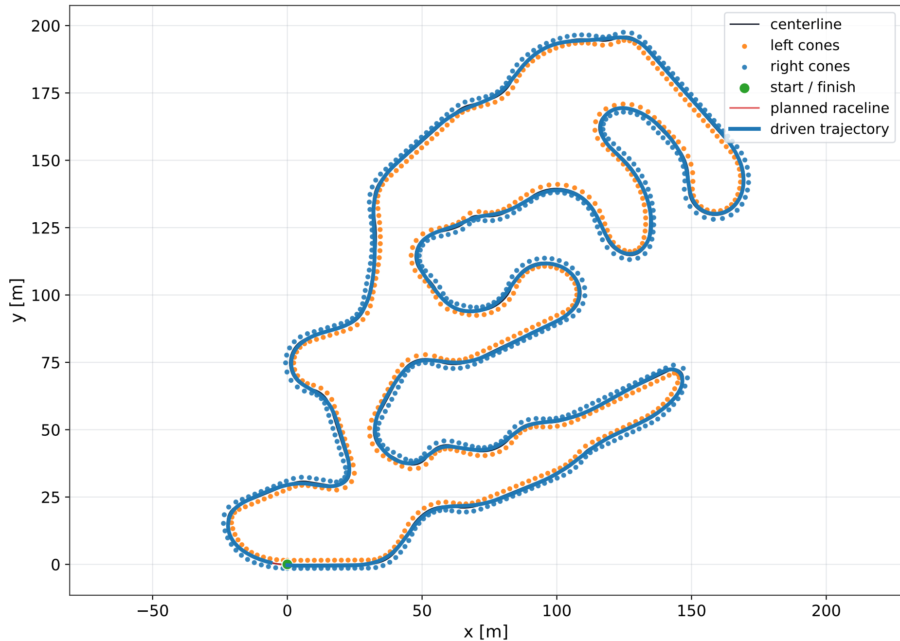
RAPP-Controlled Lap: 101.00 s, 0 incidents
