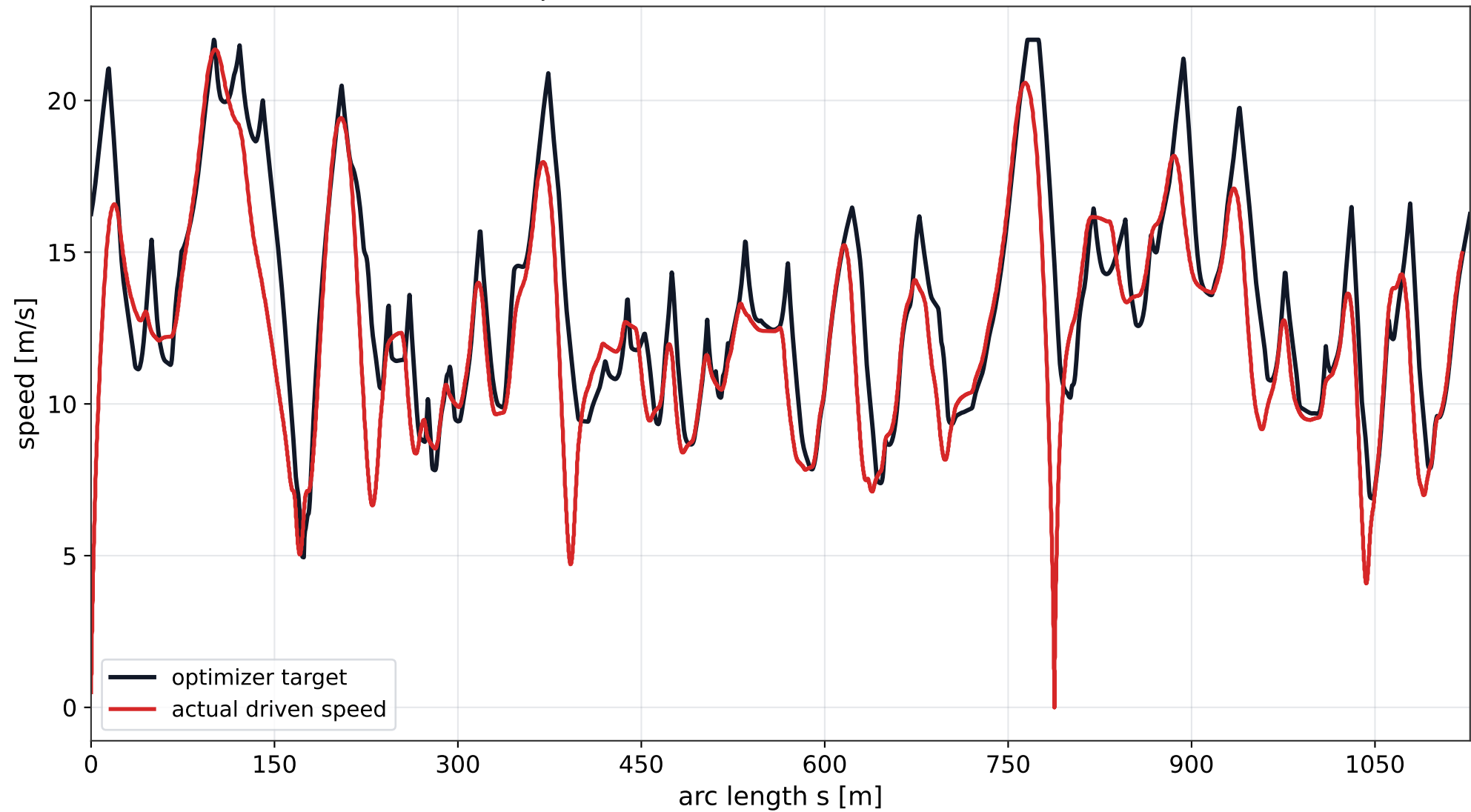
Speed Profile: Planned vs Achieved
