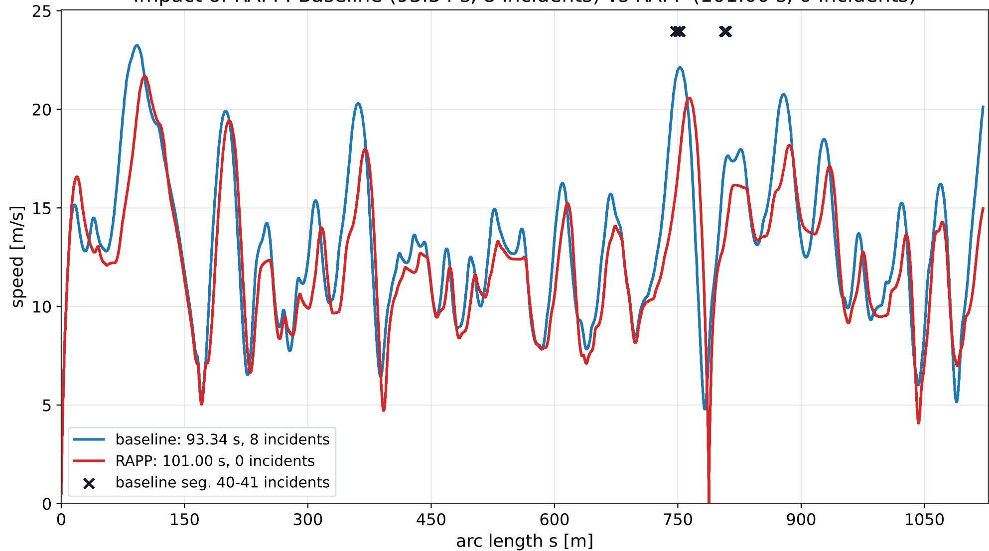
Impact of RAPP: Baseline (93.34 s, 8 incidents) vs RAPP (101.00 s, 0 incidents)
