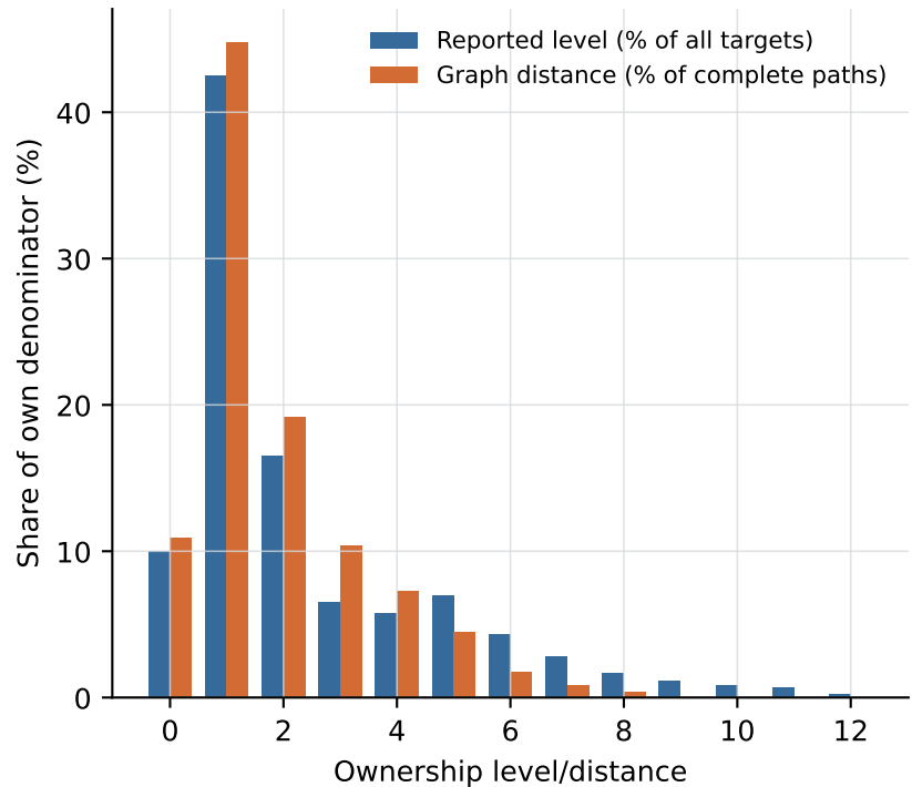
b. Reported depth is not observed graph distance
