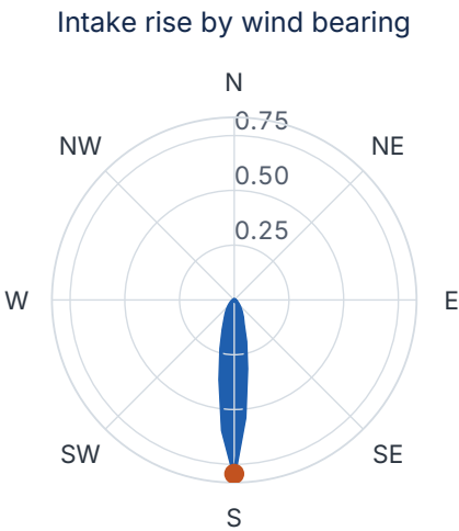
worst 0.79 °C at 180°, from 576 solves
