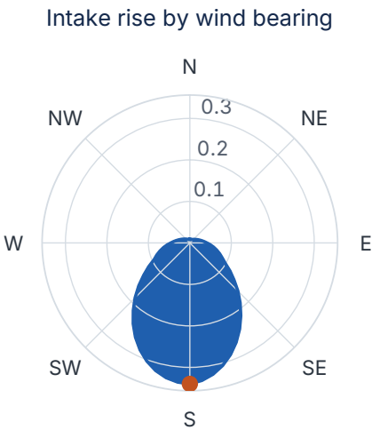
worst 0.34 °C at 180°, from 576 solves
