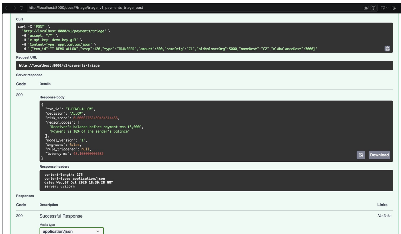
Figure 8a. A normal ₹500 transfer via Swagger: very low risk score, ALLOW, 48 ms.
