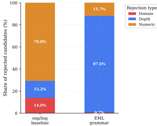
Fig. 3: Composition of rejected candidates by type. Percentages are expressed relative to the total number of rejected candidates, so the bars sum to 100% within each grammar. Under EML, depth-triggered rejections constitute 87.6% of all rejections, reflecting structural inflation as the dominant throughput constraint. Domain rejections comprise only 0.7% of EML rejections, while numeric rejections account for 11.7%. The baseline grammar shows a more balanced composition: numeric rejections (70.8%) predominate, with depth (15.2%) and domain (14.0%) rejections contributing more equally.
