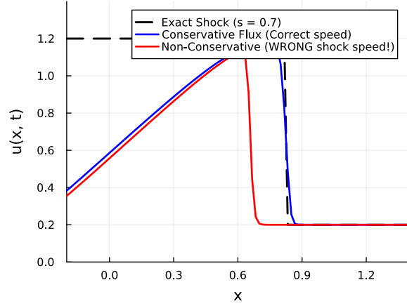
Lax-Wendroff Theorem: Shock Speed Failure
