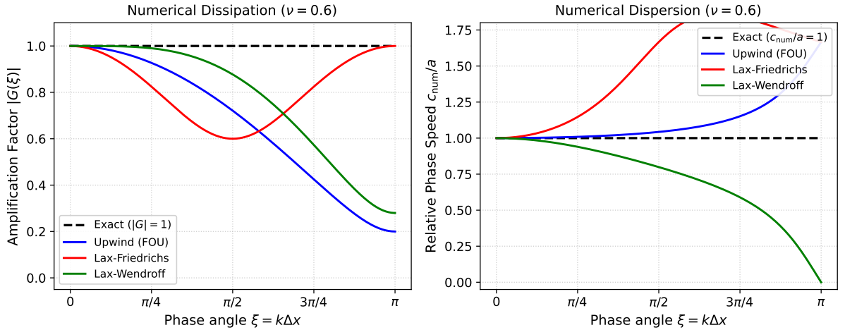
Figure 1: Left: Numerical dissipation ( |G(\xi)| vs phase angle \xi = k\Delta x for CFL \nu = 0.6 ). Right: Numerical dispersion (Relative phase velocity c_{\text{num}}/a vs \xi ).
