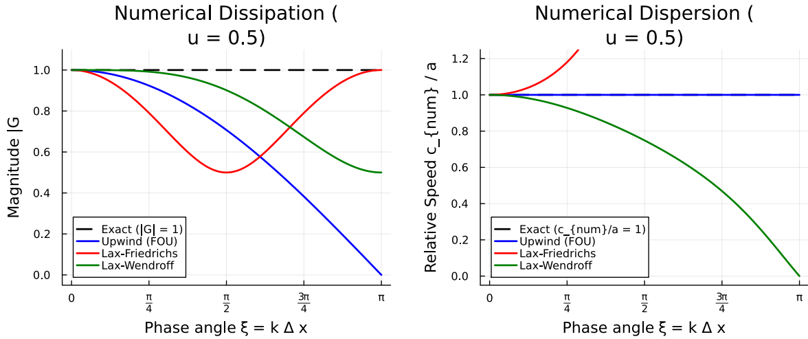
Figure 1: Left: Numerical dissipation ( |G(\xi)| vs phase angle \xi = k\Delta x for CFL \nu = 0.5 ). Right: Numerical dispersion (Relative phase velocity c_{\text{num}}/a vs \xi ). Generated with Julia.
