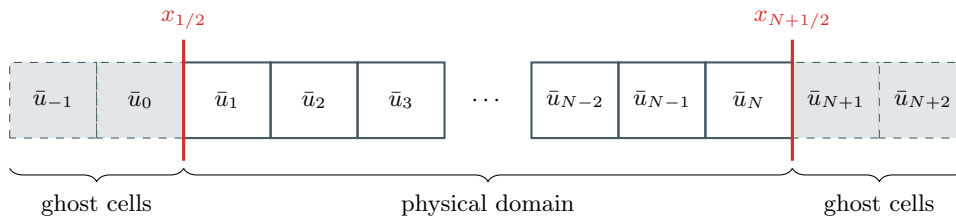
Figure 4: Two layers of ghost cells (shaded) on each side of the physical domain I_1, \dots, I_N , as required by the MUSCL stencil.
