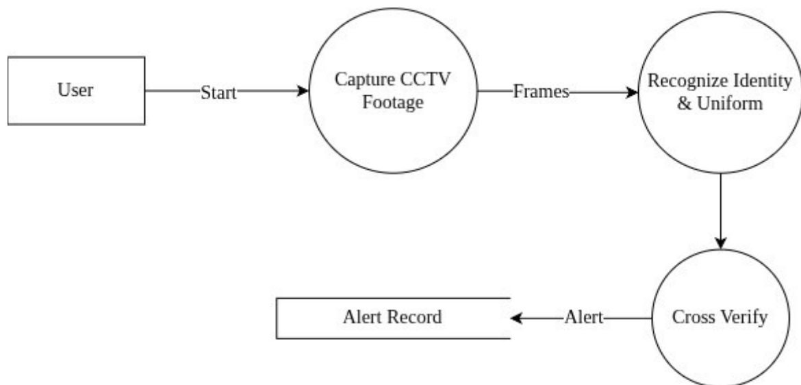
Fig-3.6.2 : Level-1 Data Flow Diagram Intelligent Surveillance and Identification for Secure Campus
