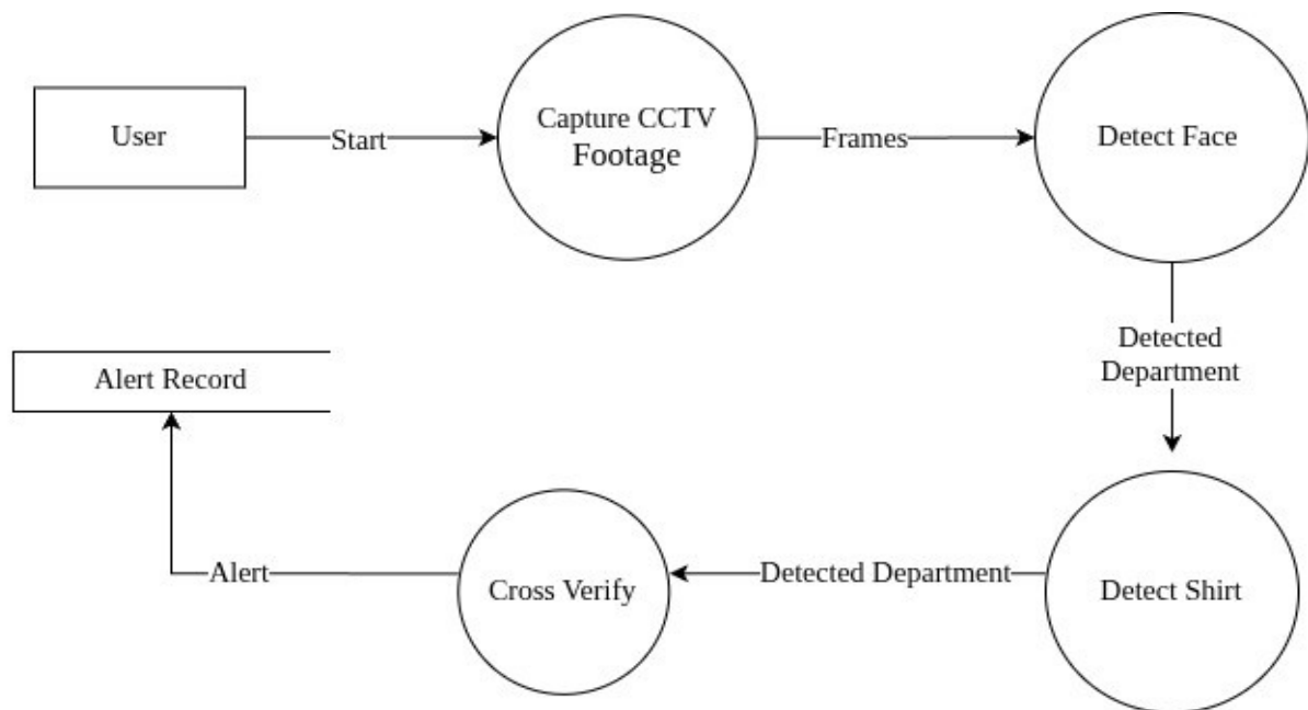
Fig-3.6.3 : Level 2 Data Flow Diagram Intelligent Surveillance and Identification for Secure Campus
