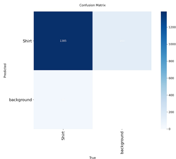
Fig-6.2: Confusion Matrix of the trained model
