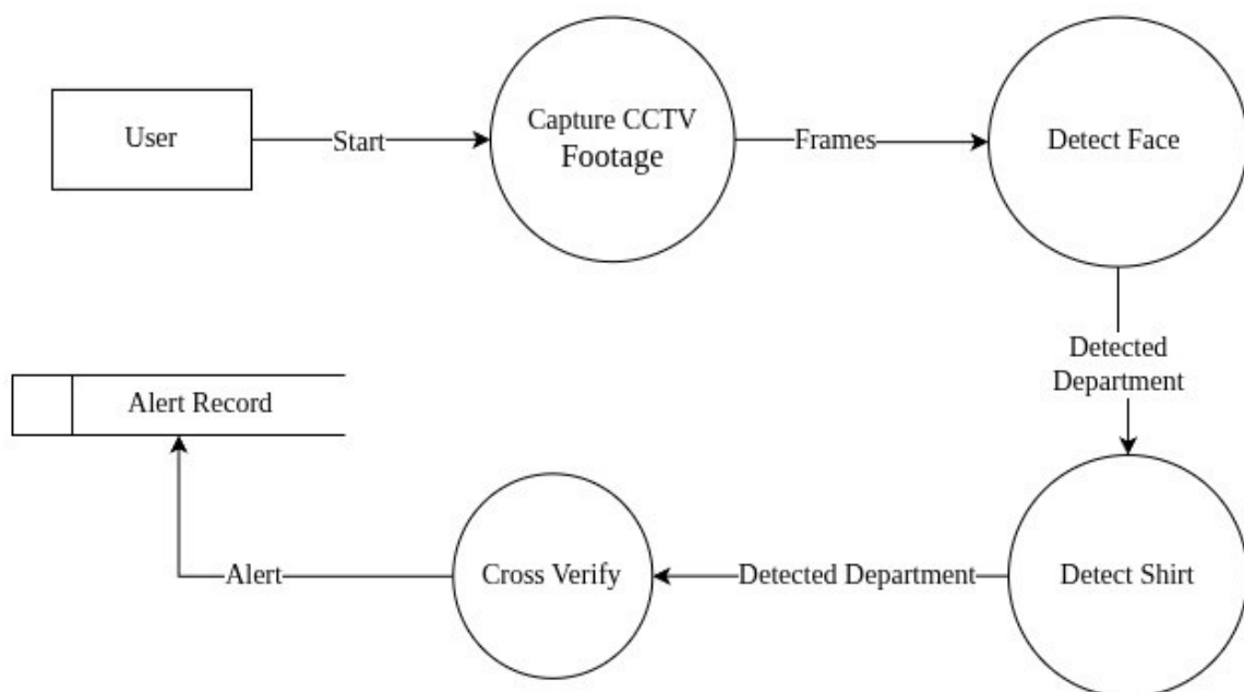
Fig-3.6.2 : Level-1 Data Flow Diagram Intelligent Surveillance and Identification for Secure Campus
