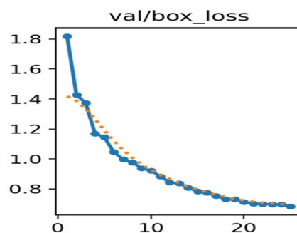
Fig-5.2 : Graph of the Loss Function of the Trained Shirt Detection Model of Intelligent Surveillance and Identification for Secure Campus
