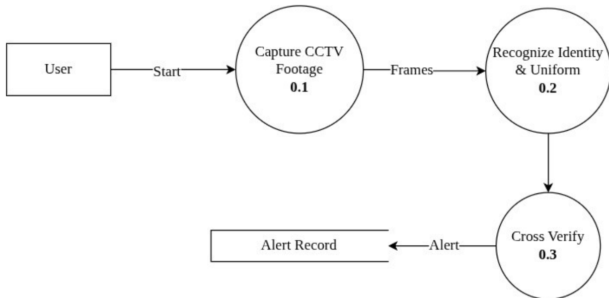
Fig-3.6.2 : Level-1 Data Flow Diagram Intelligent Surveillance and Identification for Secure Campus
