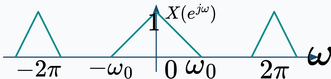
(b) 输入信号的周期频谱
